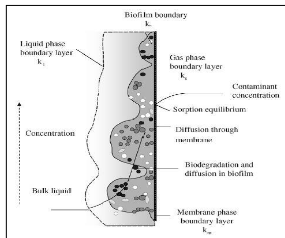
Fig 2: Mass Transfer Resistance in a Biofilm Attached on a Flat Membrane
